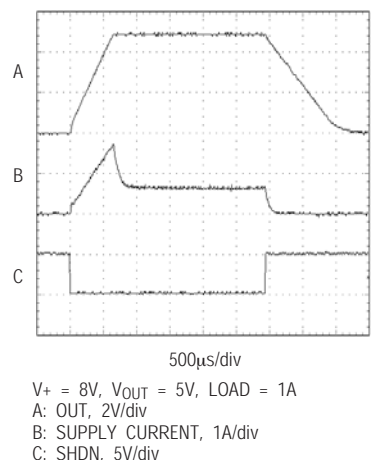
MAX1626 SHUTDOWN RESPONSE TIME AND SUPPLY CURRENT
