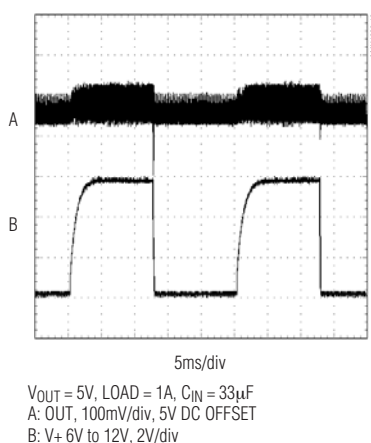
MAX1626 LINE-TRANSIENT RESPONSE
