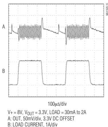
MAX1626 LOAD-TRANSIENT RESPONSE
