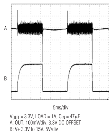
LINE-TRANSIENT RESPONSE FROM 100% DUTY CYCLE
